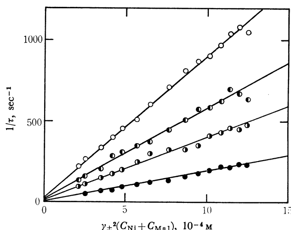
Fig. 3. 1/\tau vs. \gamma_{\pm}^2 (C_{\text{Ni}} + C_{\text{Mal}}) plot at 12°C (●), 20°C (○), 25°C (●), and 30.5°C (○).
