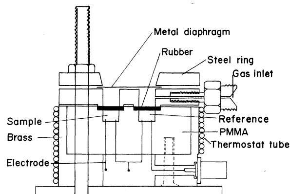
Fig. 1. Pressure-jump cell.
